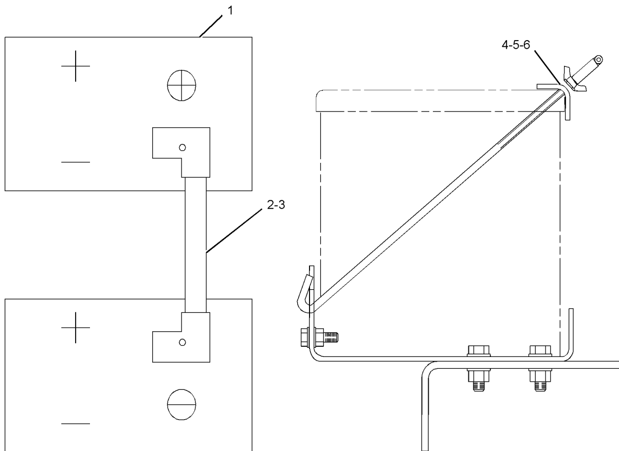
(CONNECTION DIAGRAM)
